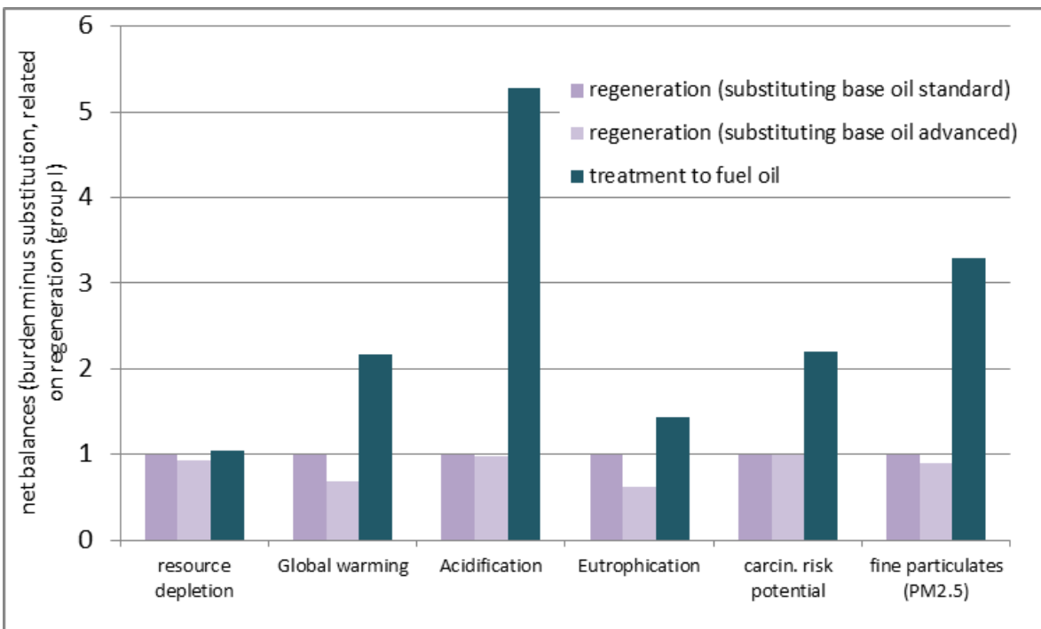
Fig. 2: Total view on the comparable impact assessment results – regeneration (average) vs. treatment to fuel; values <1 describe better performance than regeneration (base oil group I) and vice versa.
